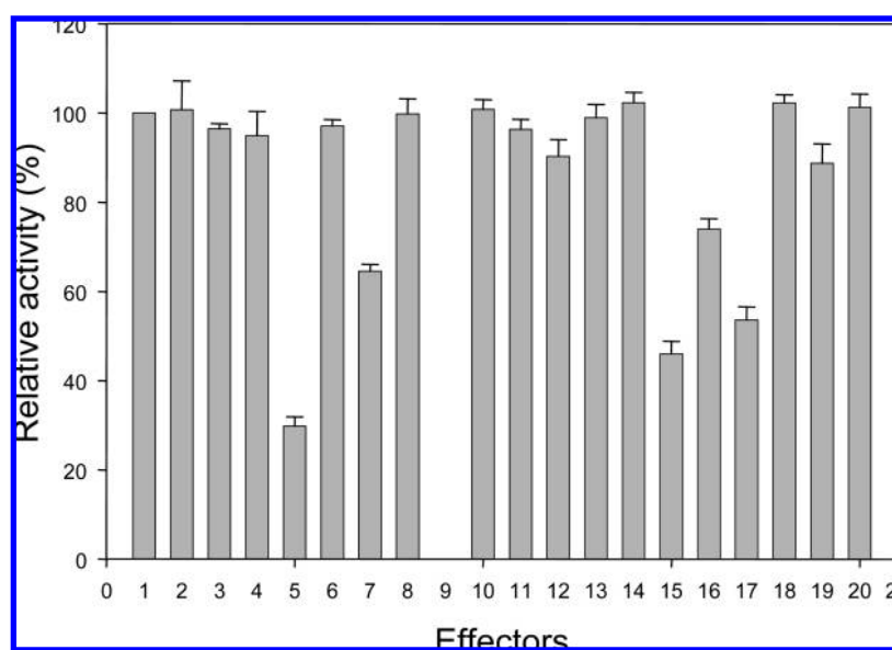
Figure 5. Effect of EDTA (2); MgCl_2 (3); iodoacetamide (4); AgNO_3 (5); NaCl (6); SDS (7); KCl (8); CuSO_4 (9); CaCl_2 (10); \beta -mercaptoethanol (11); raffinose (12); maltose (13); sucrose (14); melibiose (15); D-glucose (16); D-galactose (17); D-mannose (18); lactose (19); stachyose (20) on D. hansenii UFV-1 intracellular \alpha -galactosidase, and (1) without effectors. The final concentration of all effectors was 2 mM.
