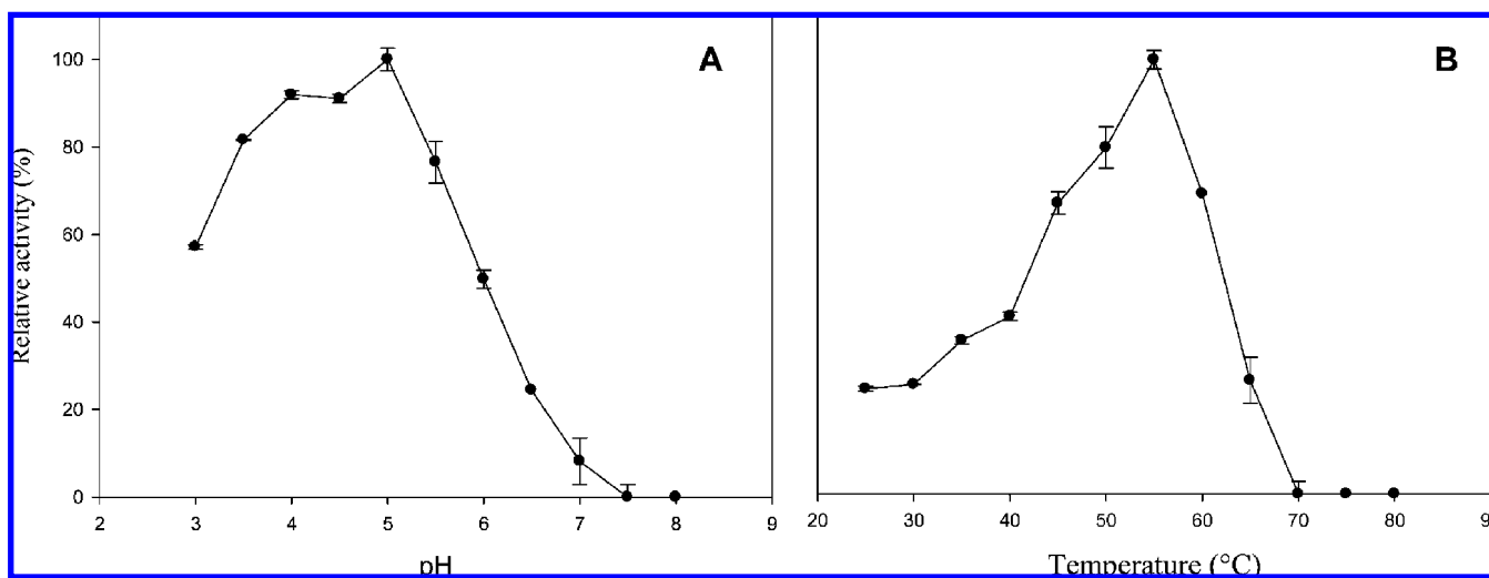
Figure 3. pH (A) and temperature (B) effects on the activity of the D. hansenii UFV-1 intracellular \alpha -galactosidase.
