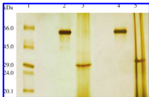
Figure 2. SDS-PAGE (12.5%) of purified and deglycosylated D. hansenii UFV-1 \alpha -galactosidases. Lane 1: molecular mass standards. Lane 2: native extracellular enzyme. Lane 3: deglycosylated extracellular enzyme. Lane 4: native intracellular enzyme. Lane 5: deglycosylated intracellular enzyme. Protein gel was stained with silver nitrate (19).
