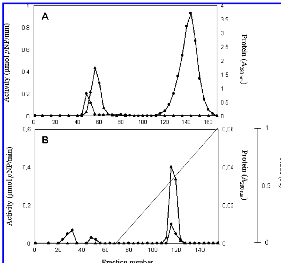
Figure 1. Elution profile of the intracellular \alpha -galactosidase from D. hansenii UFV-1 on a Sephadex G-150 column (A) and DEAE-Sepharose column (B). \alpha -Galactosidase activity ( \blacktriangle ); protein ( \bullet ) and NaCl gradient (—).
