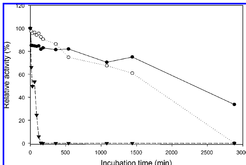
Figure 4. Effect of temperature on the stability of the D. hansenii UFV-1 intracellular \alpha -galactosidase. Enzyme preparations were preincubated for 48 h at 40 °C (●); 55 °C (○) and 65 °C (▼).
